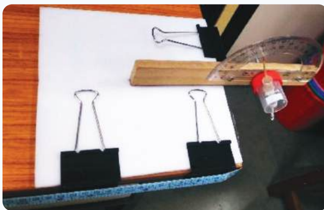
Figure 4. Top view of the launching arrangement.
